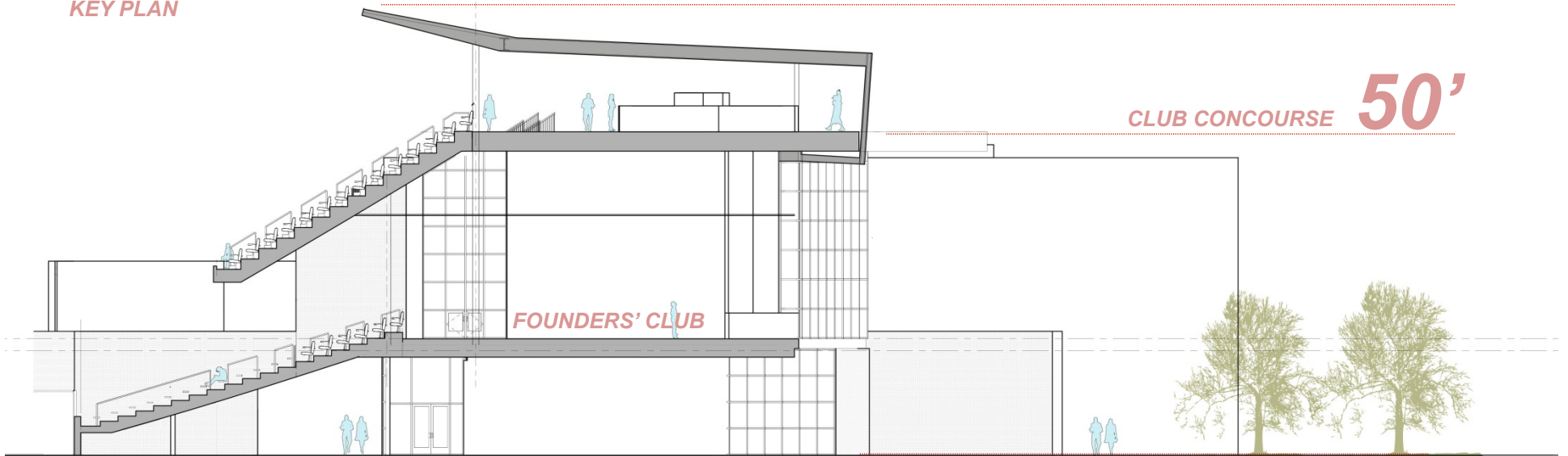
EAST SECTION AT ENTRY PLAZA
